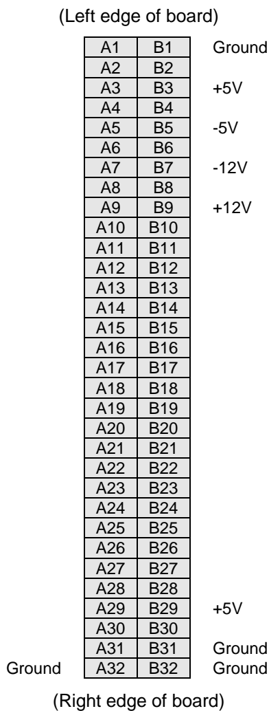
J1: PC/104 16-bit bus connector
